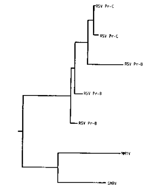
Fig. 3. Parsimonious tree of MMTV, SMRV, and two strains of RSV
