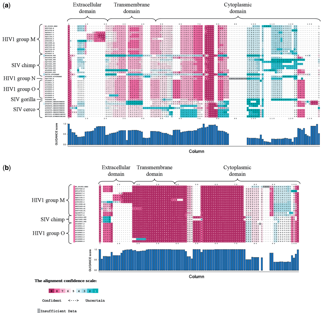
Figure 1. An example of the GUIDANCE output. (a) Residue confidence scores are projected onto the MAFFT alignment of Vpu protein sequences from human and simian immunodeficiency viruses (HIV and SIV). Confidently aligned residues are colored in shades of magenta and pink, while uncertain residues are colored in shades of blue. Column scores are plotted below the alignment. (b) Dramatically improved alignment confidence after filtering low-scoring sequences and re-running GUIDANCE. Note the color-coding next to the sequence names before and after re-alignment.
